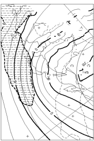
850hPa TEMPERATURE AND ANOMALY
