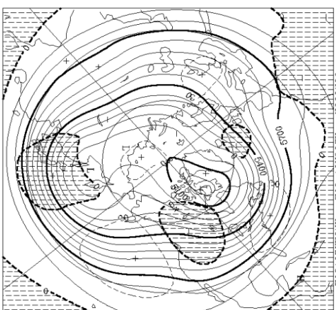
1 MONTH MEAN ( 2/ 1- 2/28 ) N:51 500hPa HEIGHT AND ANOMALY
