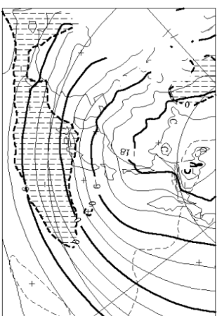
850hPa TEMPERATURE AND ANOMALY
