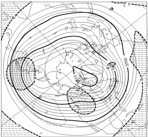
3 MONTH MEAN ( 1/ 1- 3/31 ) N:51 500hPa HEIGHT AND ANOMALY
