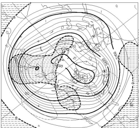
1 MONTH MEAN ( 1/ 1- 1/31 ) N:51 500hPa HEIGHT AND ANOMALY
