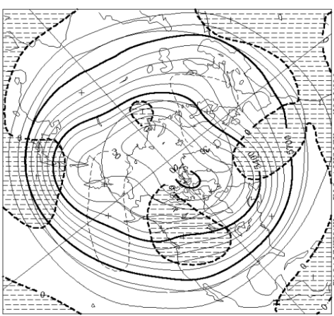
1 MONTH MEAN ( 3/ 1- 3/31 ) N:51 500hPa HEIGHT AND ANOMALY
